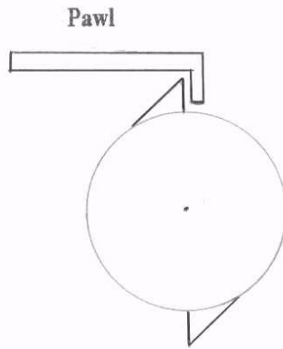
PAWL AND RATCHET WHEEL ONE WAY MECHANISM
