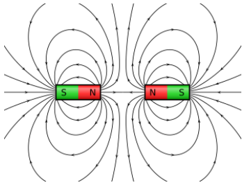
Figure 20. Opposing poles of magnets repel and push apart (They feel like elastic wave like impingement). Wikipedia (Public Domain)
