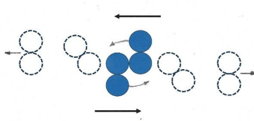
Figure 3. Similar to (Figure 2). The collision of two off-center dumbbells in the absence of a barrier. How two opposing beams of light can appear to pass directly through one another. The dumbbells rotate around their centers. Shown is a two-dimensional representation. A 3D net is required for full representation. https://youtu.be/-vCaMZ_b-w
