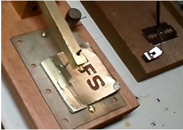
Metalized Match Book Cover and a Razor Blade Diode Detector
