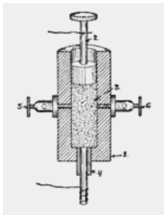
Branly's Coherer
