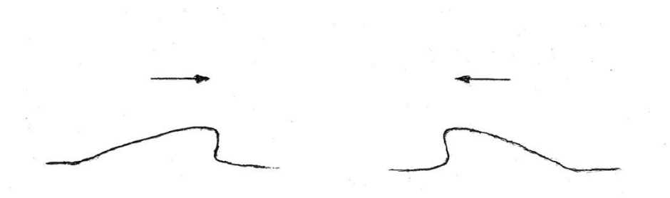
Figure 4456. Wrong. The sand patterns left by the collision of two small-sized water waves traveling in opposing directions are NOT part of the phenomenon. The collision temporarily stops the water flow motion allowing the suspended particles to drop in place creating a fake occurrence of the phenomenon.
